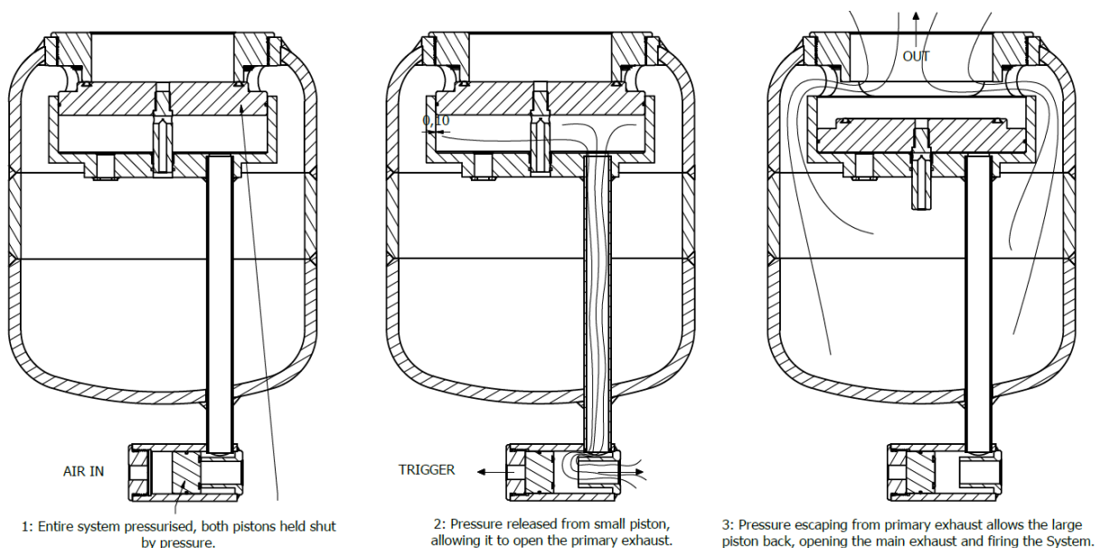
Figure 2 Cross section of the System in three phases of operation - illustrating the Operation
