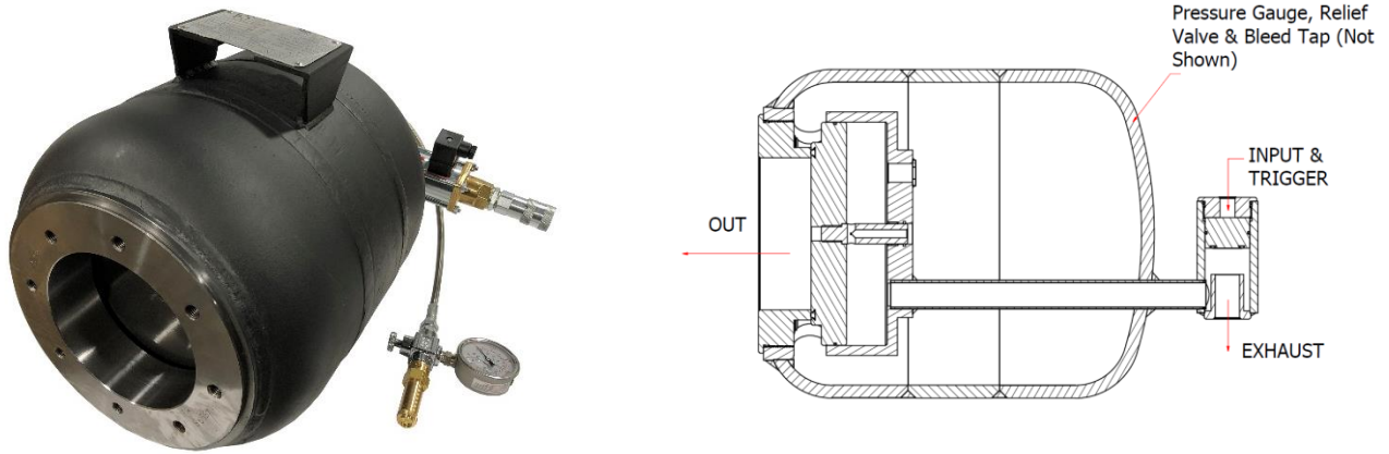
Figure 1 Air Mortar and Section through Air Chamber
