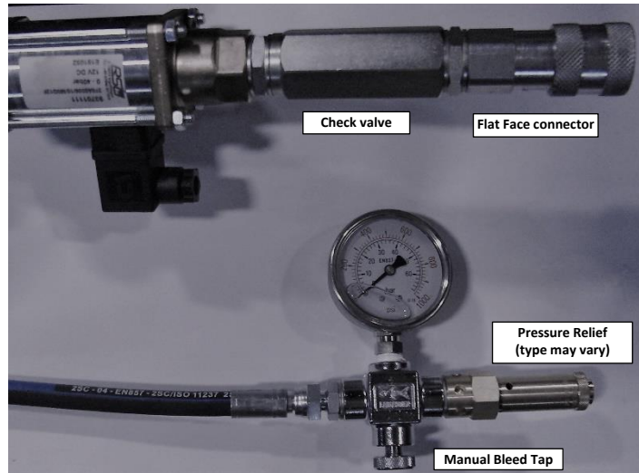
Figure 6 Detail showing: Flat Face, Check Valve & Pressure Gauge, Pressure Relief Valve and Bleed Tap
