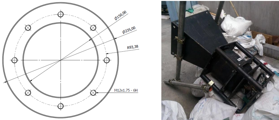
Figure 3 Output Interface and example of assembled with Snoot
